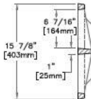
GRATE SECTION
