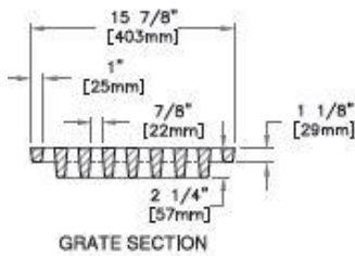
GRATE SECTION
